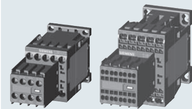
3RT Safety Contactors and 3RH Safety Control Relays
