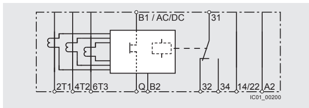
3RR2241-1F.30
